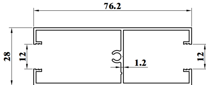
SSD753G WEIGHT : 0.725 KG/M AP : 453.76mm
