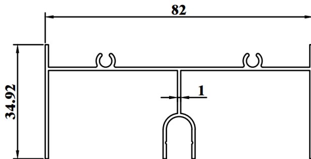
SSD745C WEIGHT : 0.580 KG/M AP : 422.43mm
