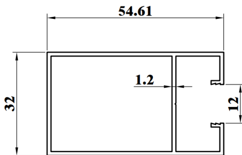
SSD754G WEIGHT : 0.619 KG/M AP : 250.85mm
