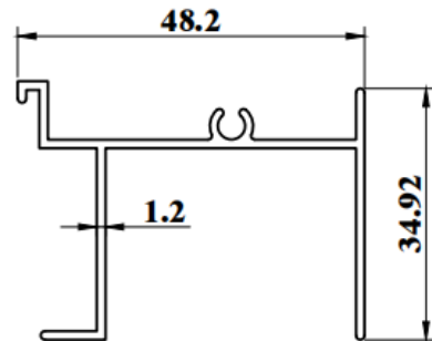
SSD746G WEIGHT : 0.438 KG/M AP : 268.32mm
