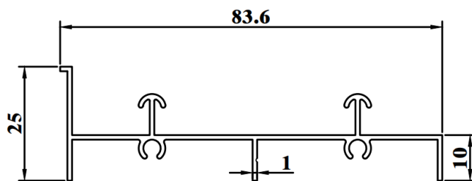
SSD747C WEIGHT : 0.477 KG/M AP : 344.24mm
