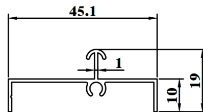
SSD748C WEIGHT : 0.239 KG/M AP : 174.31mm
