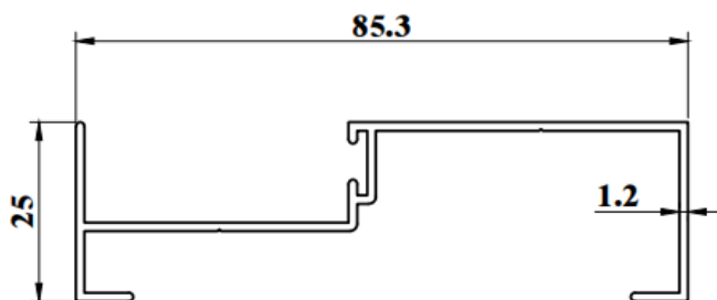
SSD749G WEIGHT : 0.540 KG/M AP : 333.58mm
