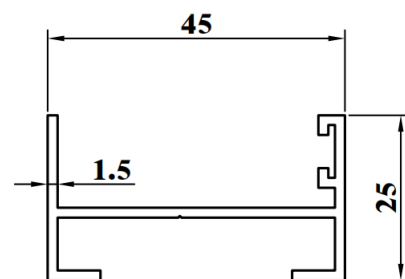
SSD750K WEIGHT : 0.459 KG/M AP : 229.21mm
