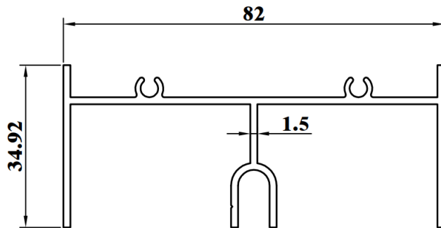
SSD745K WEIGHT : 0.840 KG/M AP : 419.36mm
