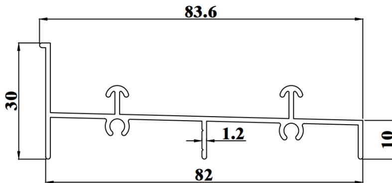
SSD796GB WEIGHT : 0.580 KG/M AP : 347.35mm
