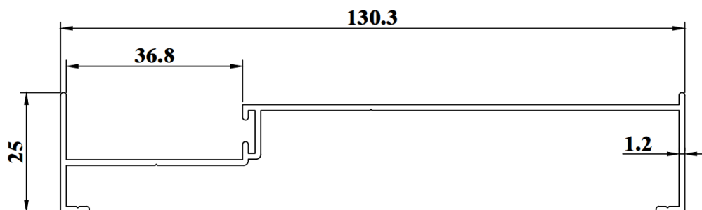
SSD791GA WEIGHT : 0.666 KG/M AP : 411.56mm
