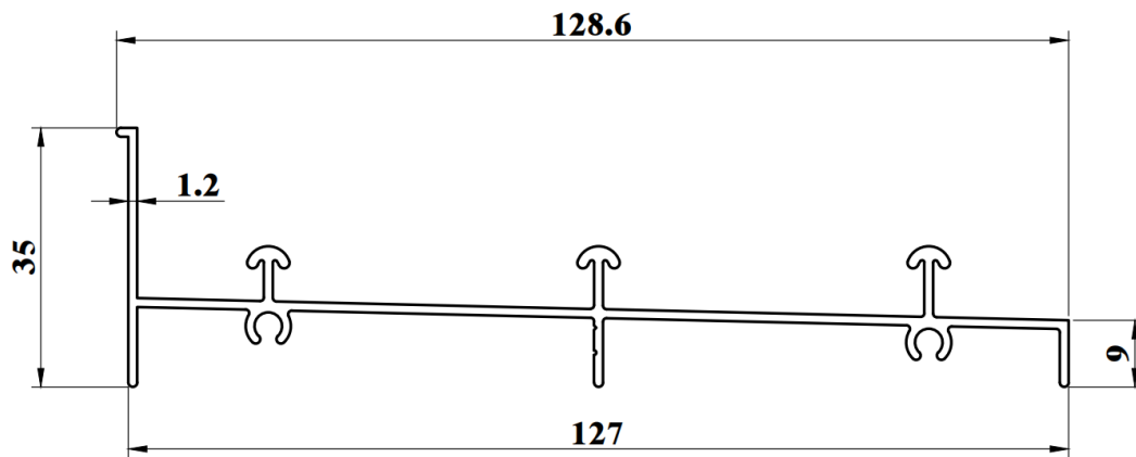
SSD792G WEIGHT : 0.805 KG/M AP : 468.96mm
