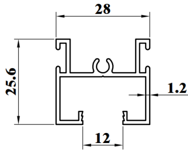
SSD751G WEIGHT : 0.380 KG/M AP : 237.07mm
