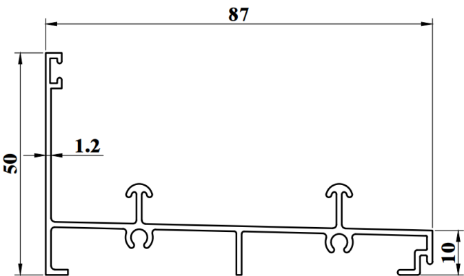
SSD916G WEIGHT : 0.731 KG/M AP : 431.86mm
