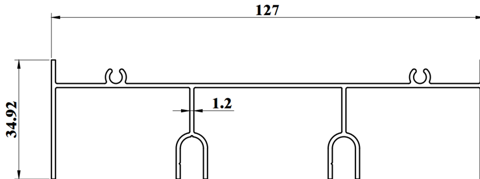
SSD786G WEIGHT : 0.980 KG/M AP : 595.64mm
