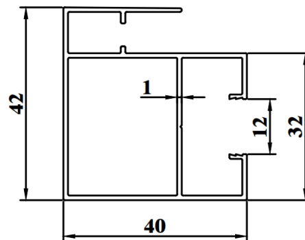
SSD752C WEIGHT : 0.542 KG/M AP : 298.83mm
