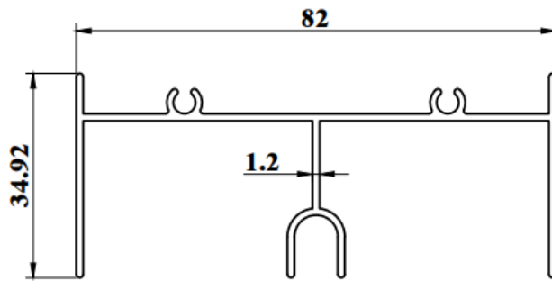
SSD745G WEIGHT : 0.679 KG/M AP : 414.13mm
