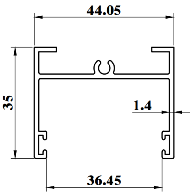
PSD788J WEIGHT : 0.546 KG/M AP : 289.86mm
