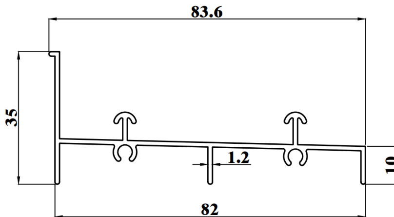
SSD796G WEIGHT : 0.595 KG/M AP : 356.86mm
