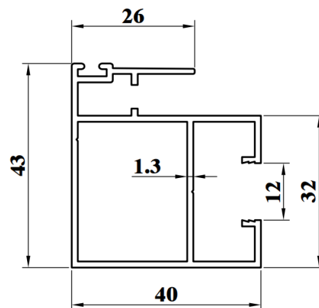
SSD752HH WEIGHT : 0.716 KG/M AP : 308.33mm
